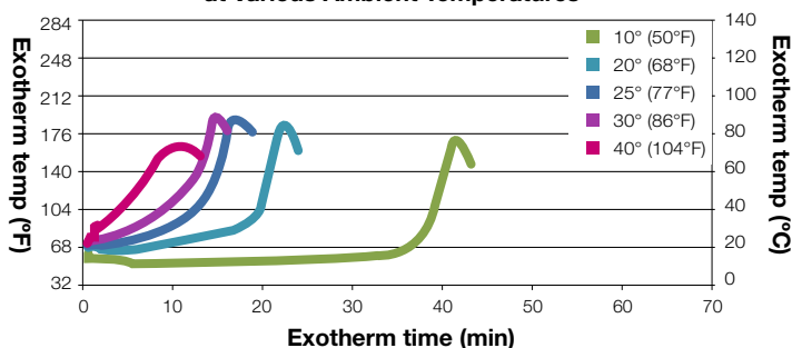
Typical Exotherm Curve for MA320 (10g mass) at Various Ambient Temperatures 5
