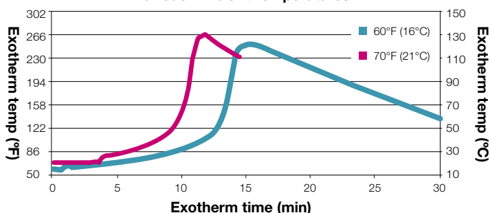
Typical Exotherm Curve for MA830 (10g mass) Various Ambient Temperatures 5
