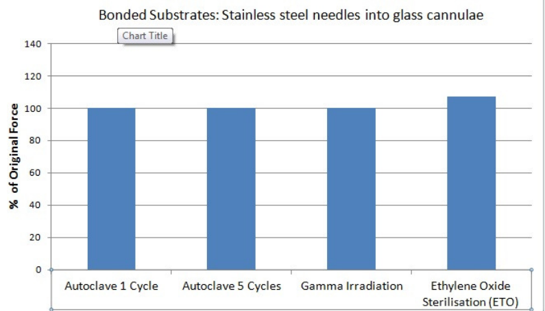
Needle Extraction Forces of Vitalit 6108 after Different Sterilisation Processes
